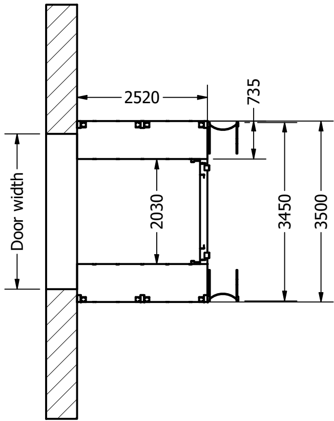
SECTION D-D SCALE 1 / 75
